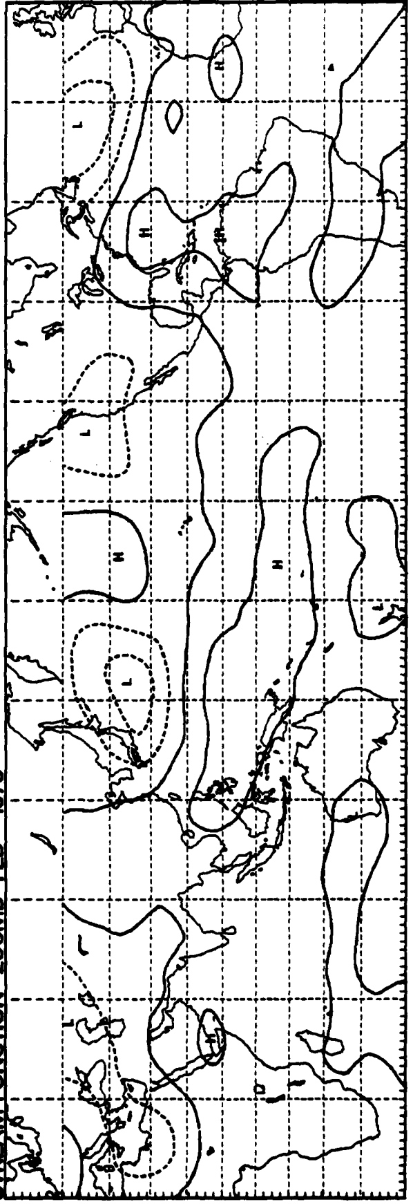
STREAM FUNCTION 200MB FEB 1975
